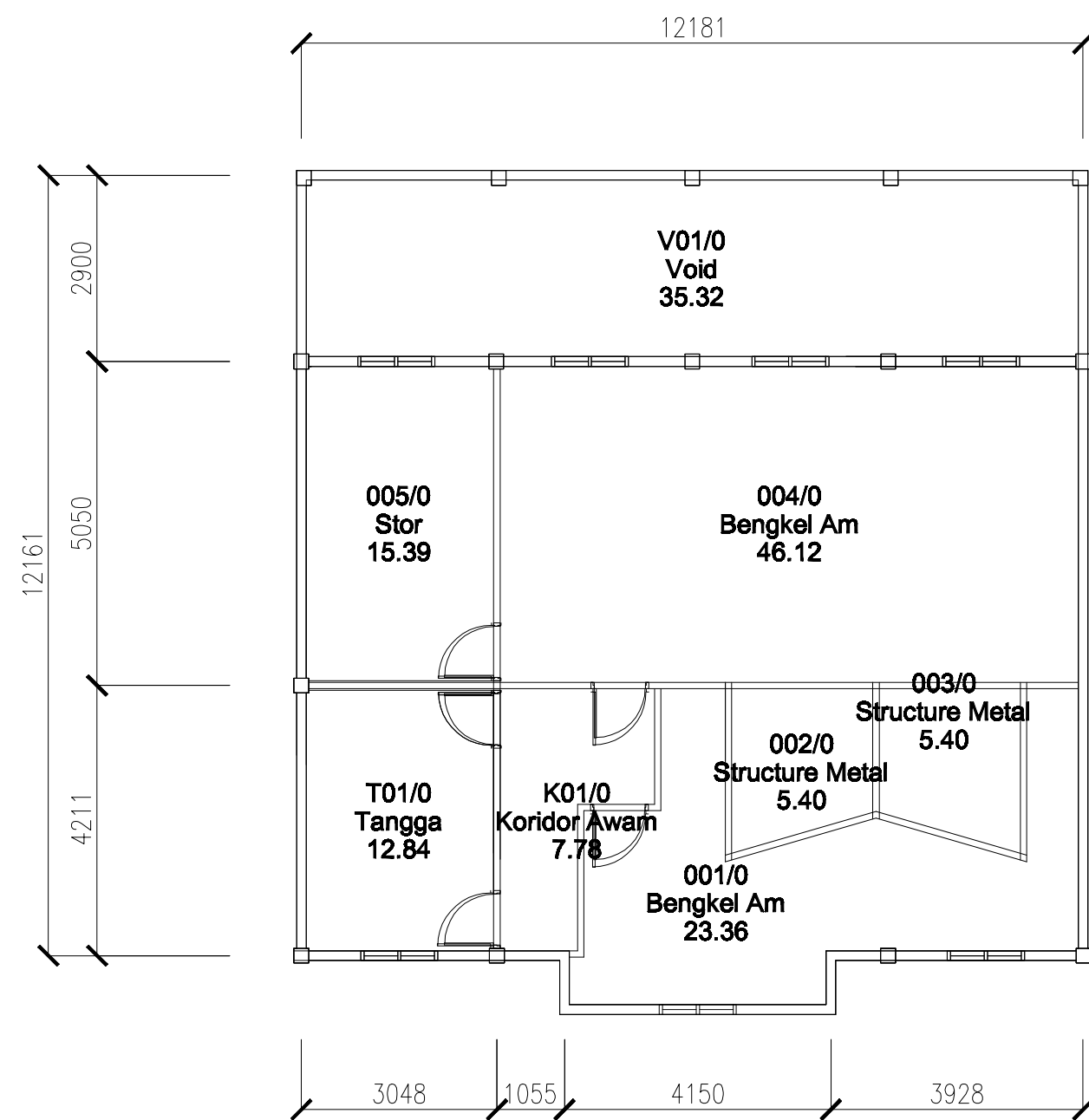
BENGKEL FSPU - ARAS 2 SCALE 1:125
